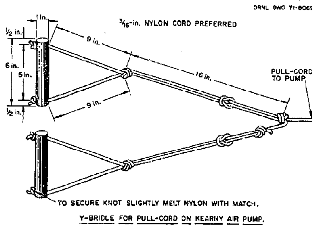
Fig. B-21. Y-bridle for pull-cord on Kearny Air Pump.
